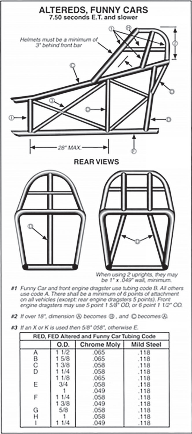
Figure 8: Altered, Funny Car roll cages
