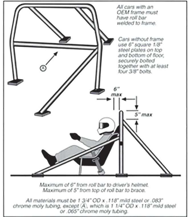
Figure 7: General roll bar specs
