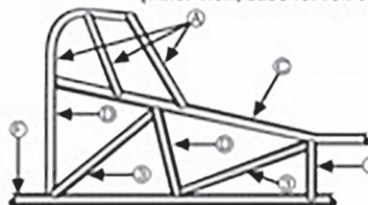
Figure 10: Street roadster roll cage
