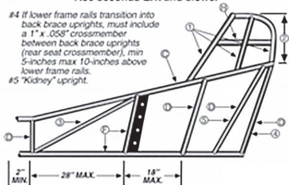
Figure 9: Rear-Engine Dragster roll cage
