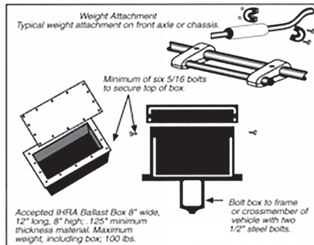
Figure 1: Ballast
