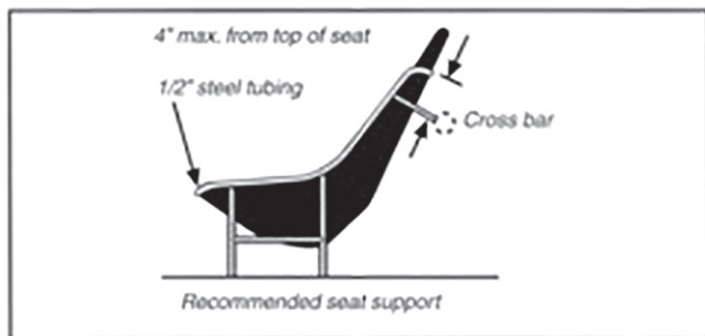
Figure 14: Seat mounting
