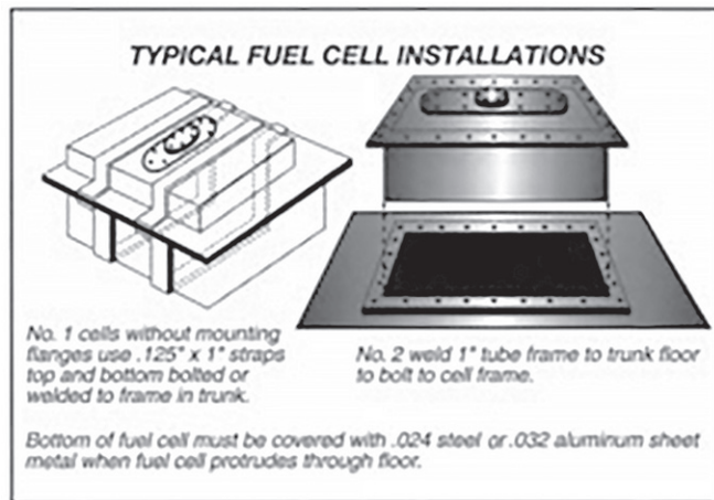
Figure 6: Fuel cell installation
