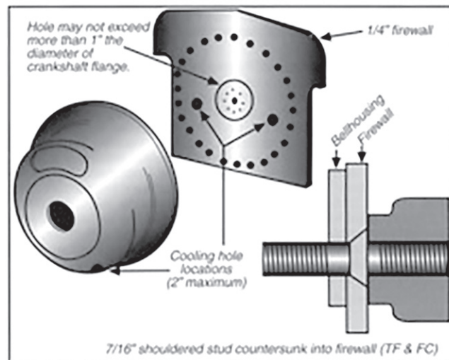
Figure 5: Motor plate
