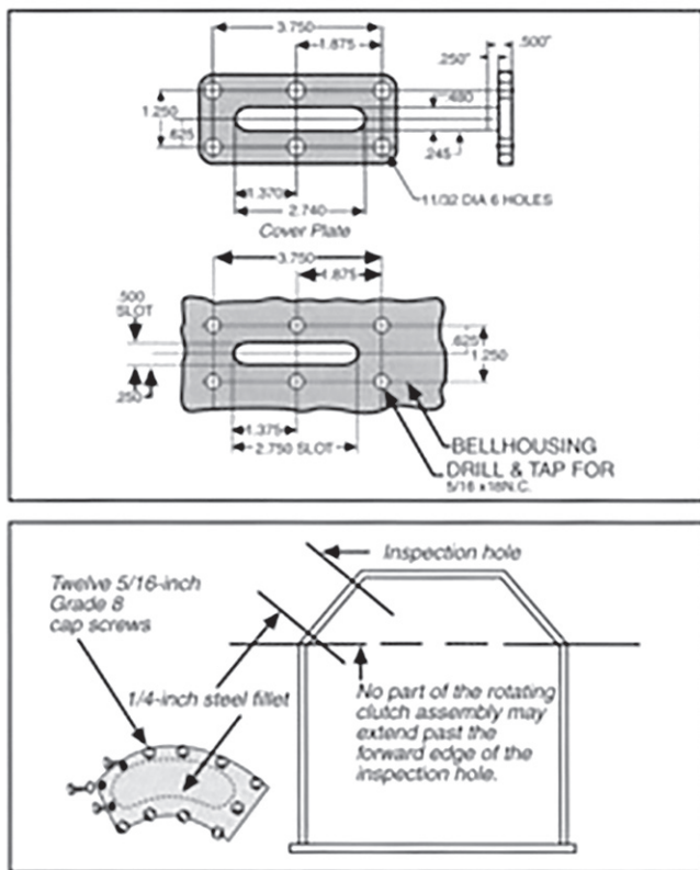
Figure 3 and 4: Bellhousing inspection hole cover
