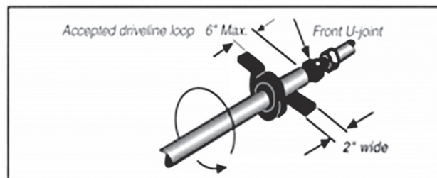
Figure 2: Driveline loop.
