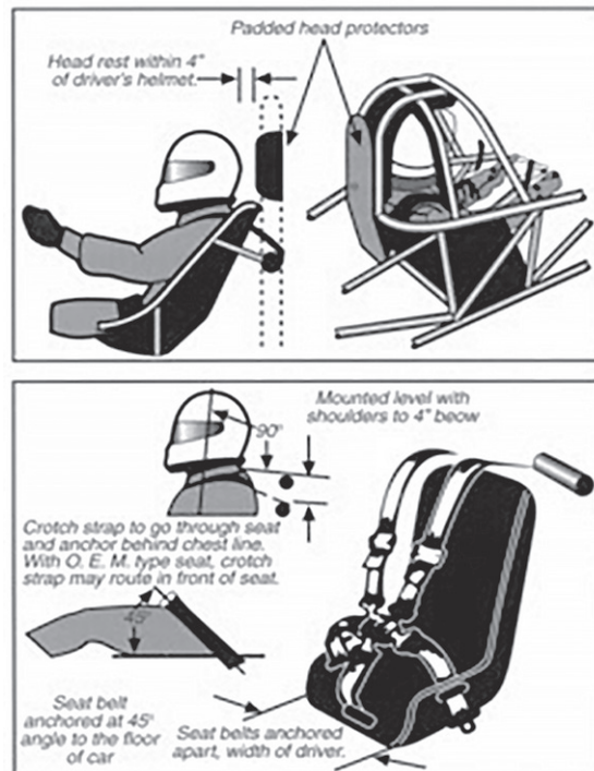
Figure 12 and 13: Head protectors and harness mounting
