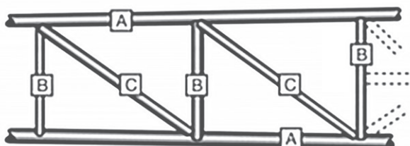
BOTTOM VIEW
